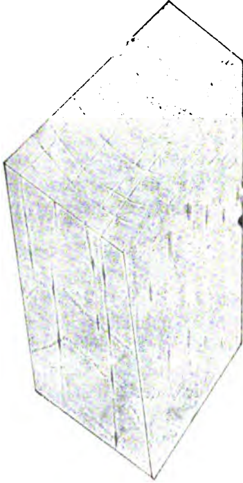
Fig. 19.—Type of Alderwood ( Alnus ).
